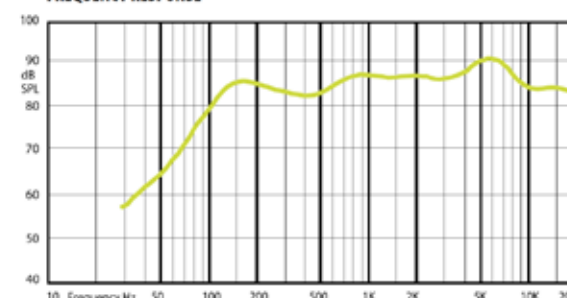
FREQUENCY RESPONSE
