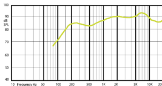
FREQUENCY RESPONSE
