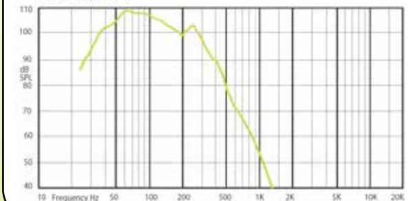
FREQUENCY RESPONSE
